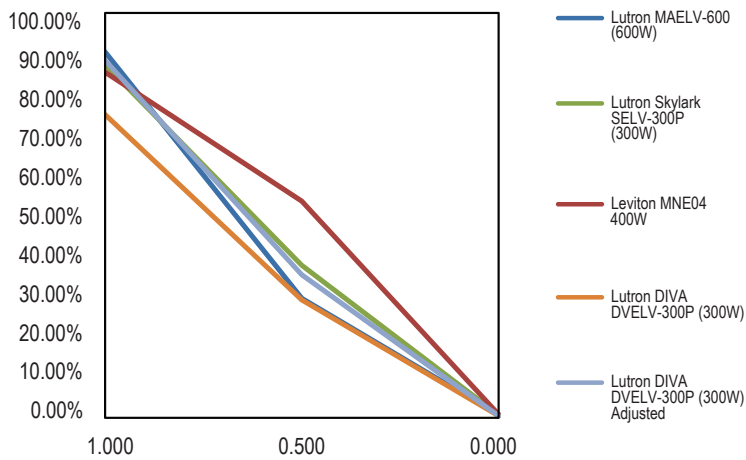
Output Current Vs Dimmer
